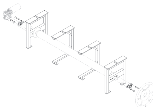
1505 UNDER BENCH ROLLER
